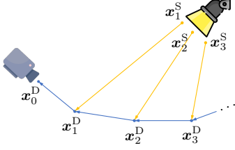
Fig. 4. With next-event estimation (NEE), a unidirectional path tracer effectively constructs a set of light paths that share one detector subpath ( \mathbf{x}_0^D, \mathbf{x}_1^D, \dots ) shown in blue. The arrows in this figure illustrates the flow of light. We present a technique to efficiently compute and differentiate the measurement contribution of all paths by factoring out common terms.
