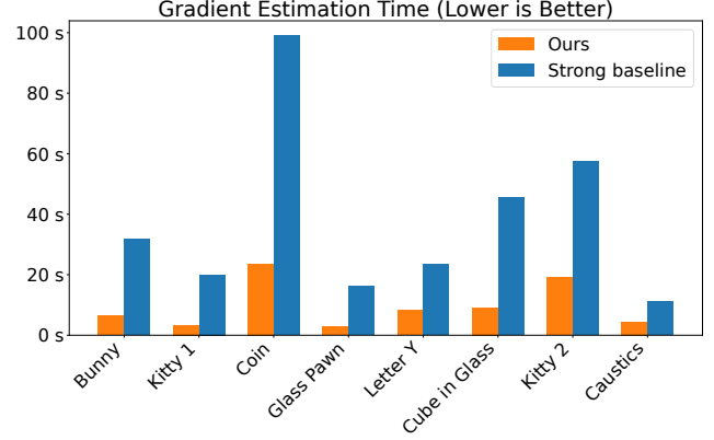
Fig. 8. Performance comparison: We compare running times for estimating image-loss gradients dL/d\theta when solving the inverse-rendering problems in Figures 9, 10, and 11. The strong baseline, which already outperforms existing CPU-based systems [Zhang et al. 2020, 2021b], uses Enzyme to differentiate full material measurement contributions \hat{f}(\mathbf{p})[r] in Eq. (15).
