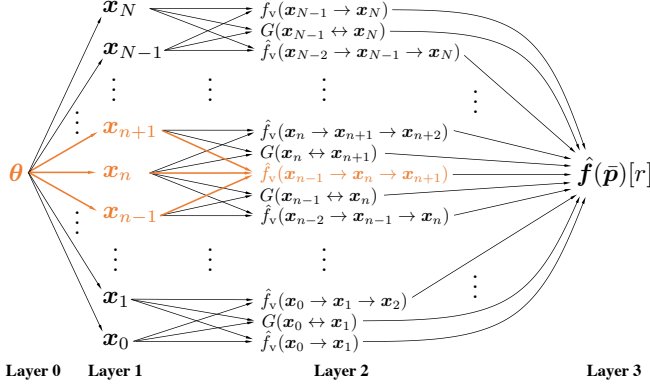
Fig. 3. A layered computation graph for evaluating the material measurement contribution \hat{f}(\bar{p})[r] . All terms on which \hat{f}_v(x_{n-1} \rightarrow x_n \rightarrow x_{n+1}) depends are highlighted in orange. We omitted the vertices p_n of the material path \bar{p} as they are independent of the scene parameters \theta .
