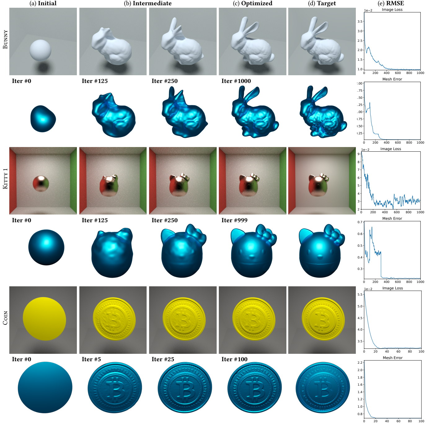
Fig. 9. Inverse-rendering results obtained with gradients estimated using our differentiable unidirectional path tracer. The mesh error plotted in column (e) captures the Chamfer distance [Barrow et al. 1977] between the reconstructed and groundtruth geometries (normalized so that the GT has a unit bounding box). We use this information only for evaluation (and not for optimization).
