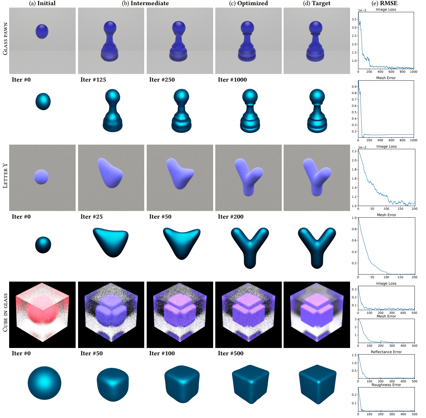
Fig. 10. Inverse-rendering results obtained with gradients estimated using our differentiable unidirectional path tracer. All examples in this figure involve non-opaque (i.e., transparent or translucent) objects that cannot be easily handled by simple rasterization-based or direct-illumination-only differentiable renderers. The mesh, reflectance, and roughness errors are used for evaluation only (and not for optimization).
