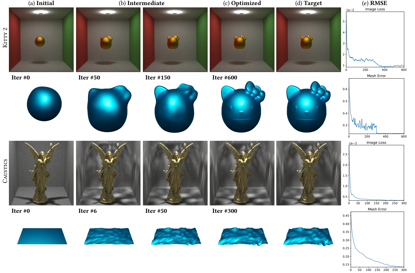
Fig. 11. Inverse-rendering results obtained with gradients estimated using our differentiable bidirectional path tracer. The mesh error is used for evaluation only (and not for optimization).
