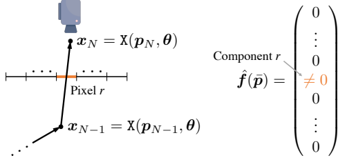
Fig. 2. Given a material light path \bar{p} = (p_0, \dots, p_{N-1}, p_N) , its material measurement contribution \hat{f}(\bar{p}) is typically very sparse where only components corresponding to pixels that “intersect” the segment \bar{x}_{N-1} \bar{x}_N —i.e., pixels whose reconstruction filters have supports covering the projection of \bar{x}_{N-1} on the image plane—are nonzero.
