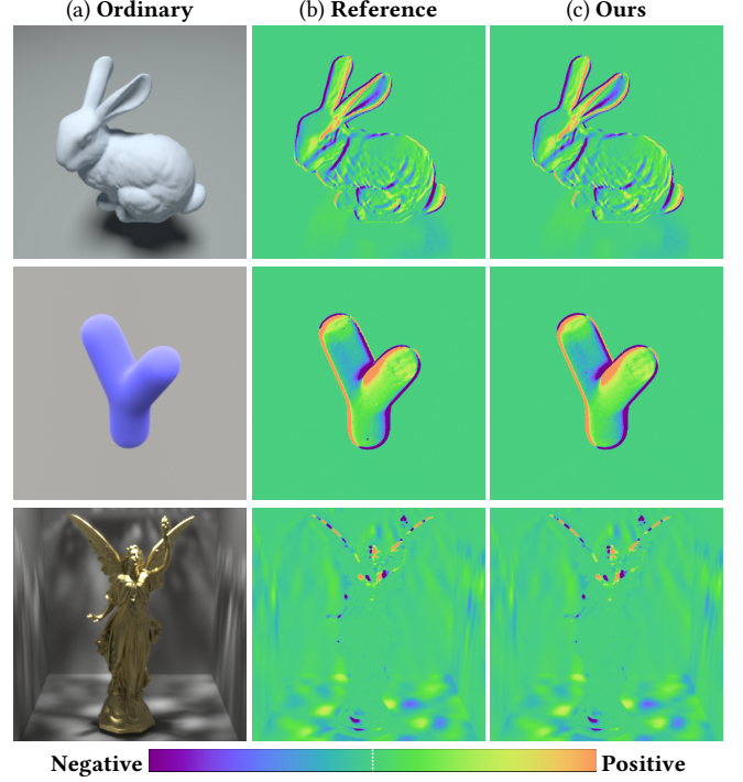
Fig. 6. We validate our system by comparing our generated gradient images with references.
