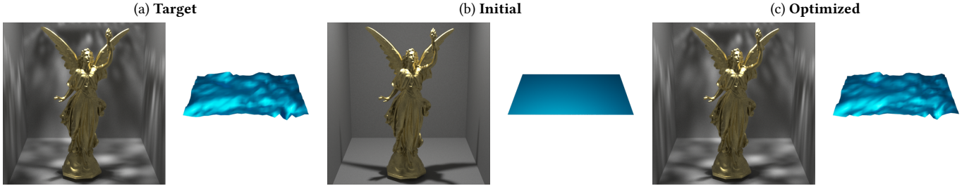
Fig. 1. We introduce a new, efficient and scalable computational differentiation technique for path-space differentiable rendering. We formulate image-loss gradients – an essential ingredient for solving inverse-rendering optimizations – as differential path integrals, before introducing new algorithms to efficiently estimate these path integrals. This example involves a underwater scene with a glossy Lucy model. We optimize the shape of the air-water interface (described using 651 mesh parameters) to match the caustics patterns. Our system improves on the generality and performance for solving inverse-rendering problems that involve both complex light transport effects and large numbers of parameters. (Using Adobe Acrobat and clicking on column (c) will play an animation of our optimization.)
